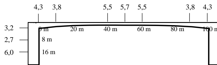
Figure 1: Reliability indexes \beta of the static proof bending under normal forces in ultimate limit state regarding a period of 50 years
