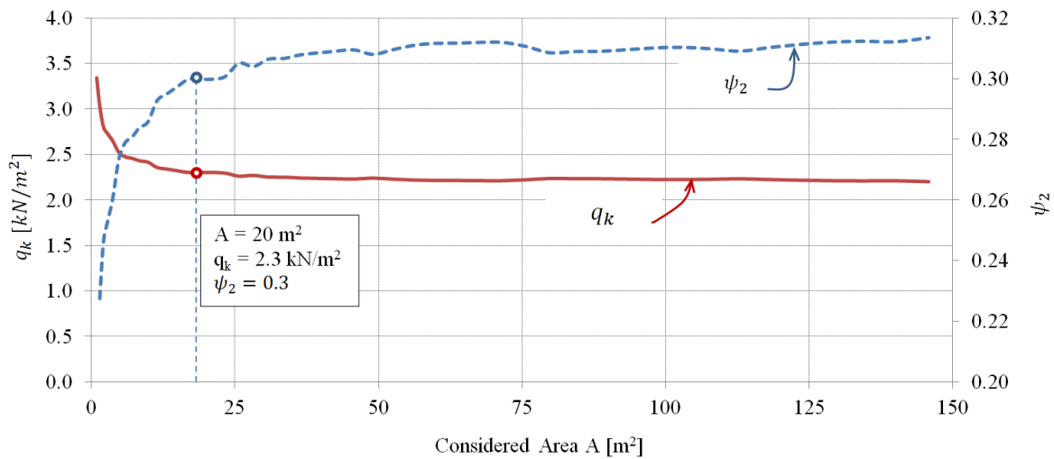
Figure 2: Characteristic distributed load q_k and load combination factor \Psi_2
