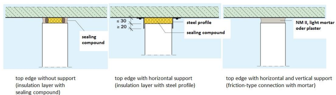
Figure 1: Supports for non-load-bearing masonry walls according to (1)
