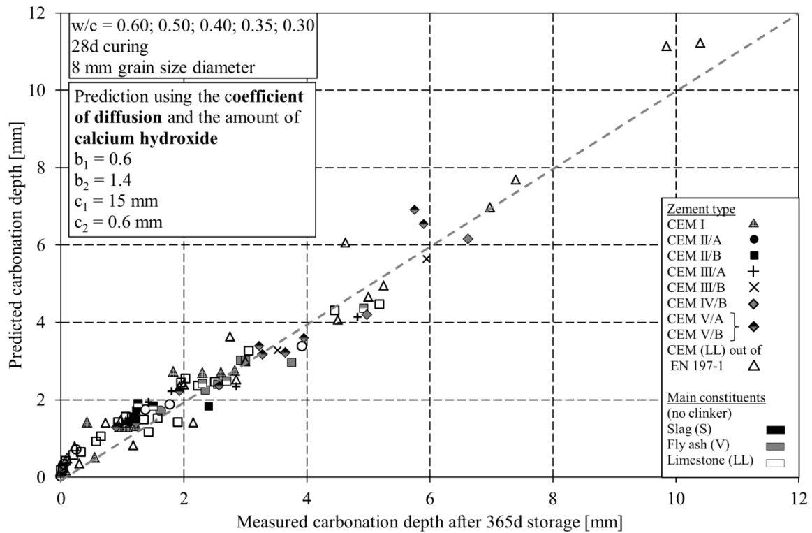
Figure 1: Comparison of measured and predicted carbonation depths
