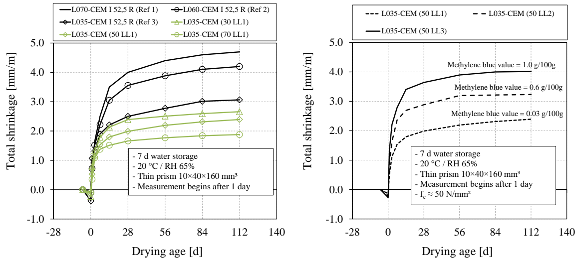
Figure 1: Shrinkage deformation of hardened cement pastes
