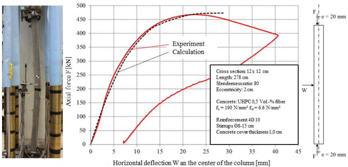
Figure 1: Experimental load bearing test (left); Stress-deformation-curve of the experimental test and the Finite-Element-Modell (right)
