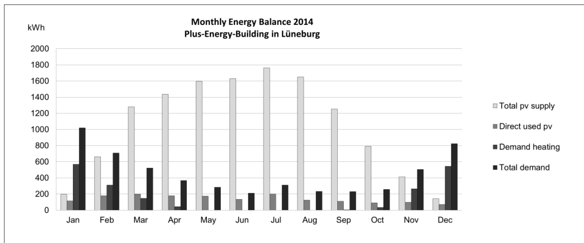
Figure 1: Monthly energy balance of the plus-energy-building in Lüneburg
