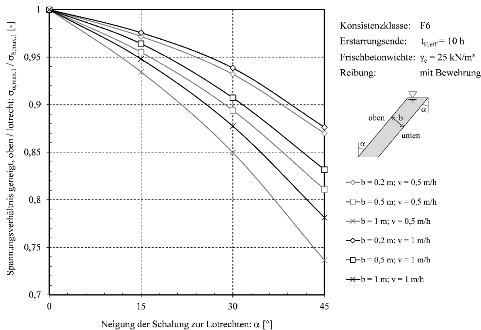
Figure 1: Pressure ratio of fresh concrete pressure of a upper inclined formwork and a vertical formwork (comp. (2))
