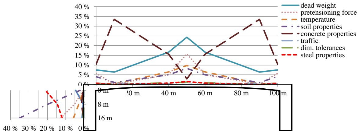
Figure 2: Basic variables of the static proof bending under normal forces in ultimate limit state without model uncertainties
