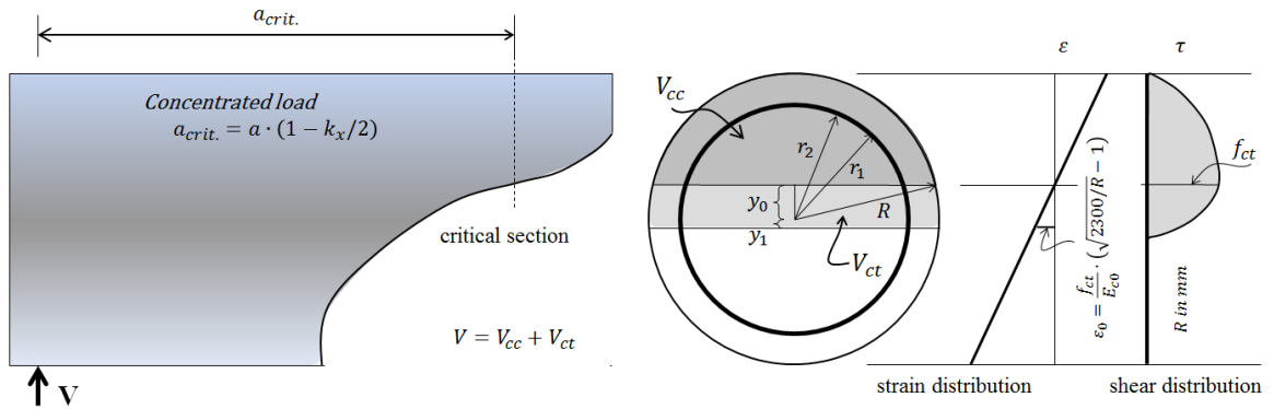
Figure 1: Shear model
